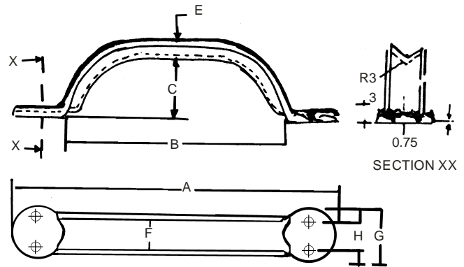
Fig. 9.12.3 : Typical Door Handle (Type 3)
