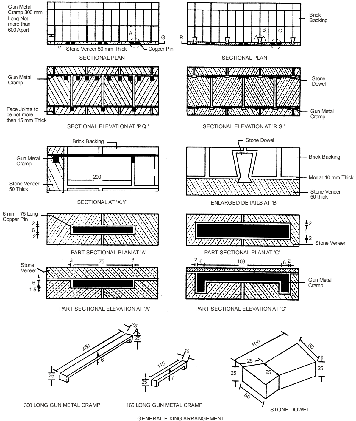
Fig. 7.14 : Stone Veneering
